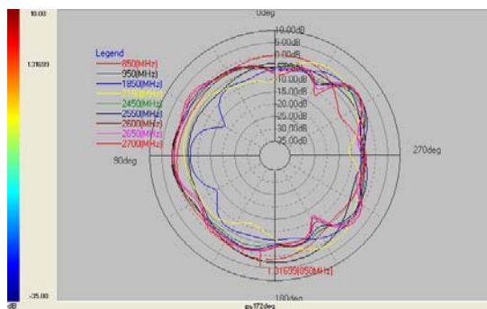
H-Plane at all Frequency
