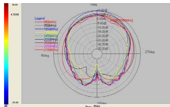
E-Plane at all Frequency
